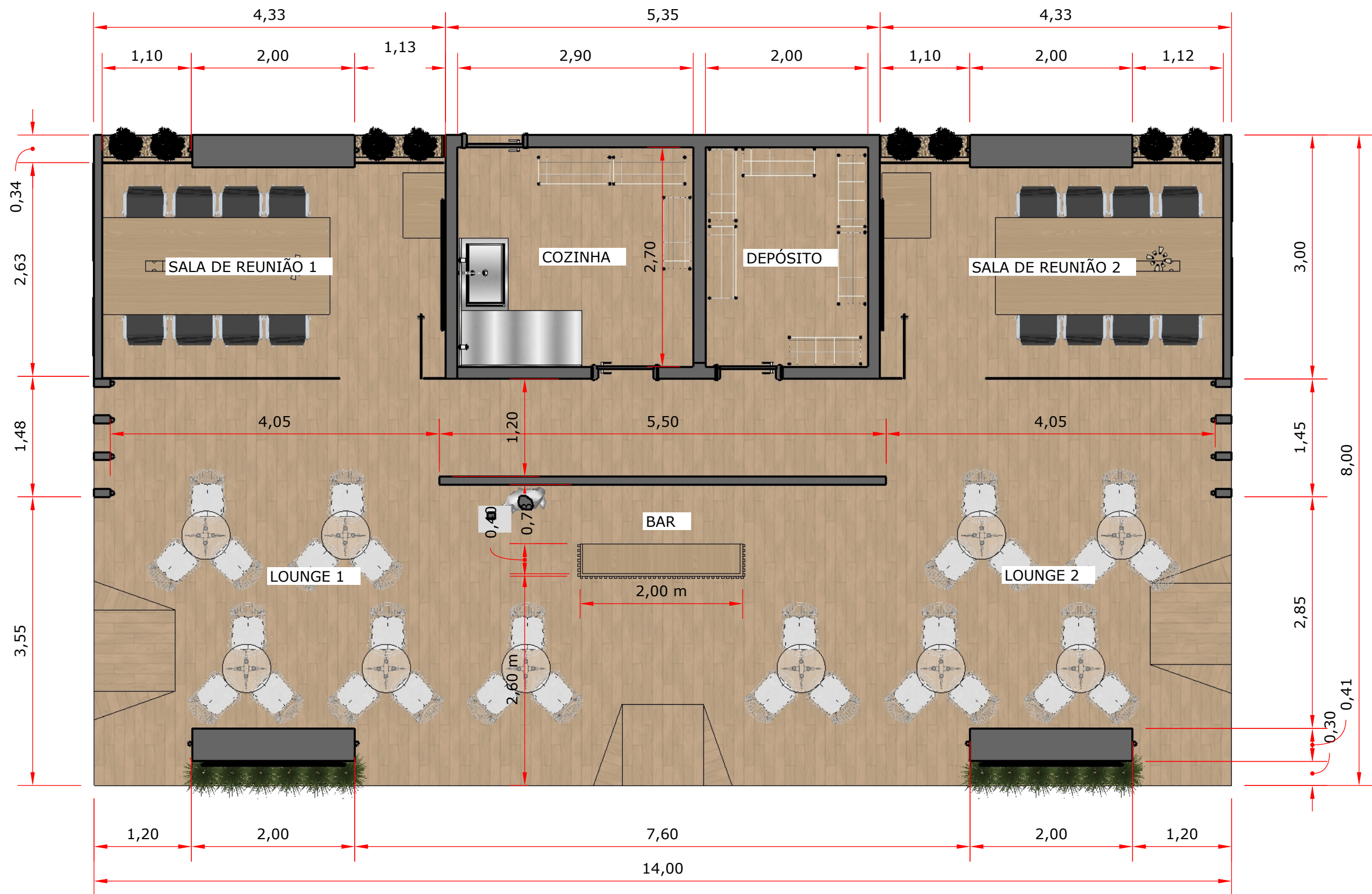
01 LAYOUT escala 1/50
